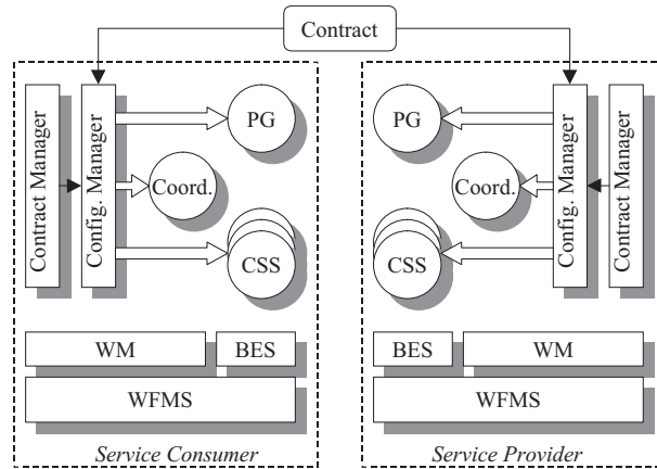
Figure 2: Infrastructure setup.
